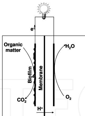
Fig. 3. Microbial Fuel Cell (MFC) set up
